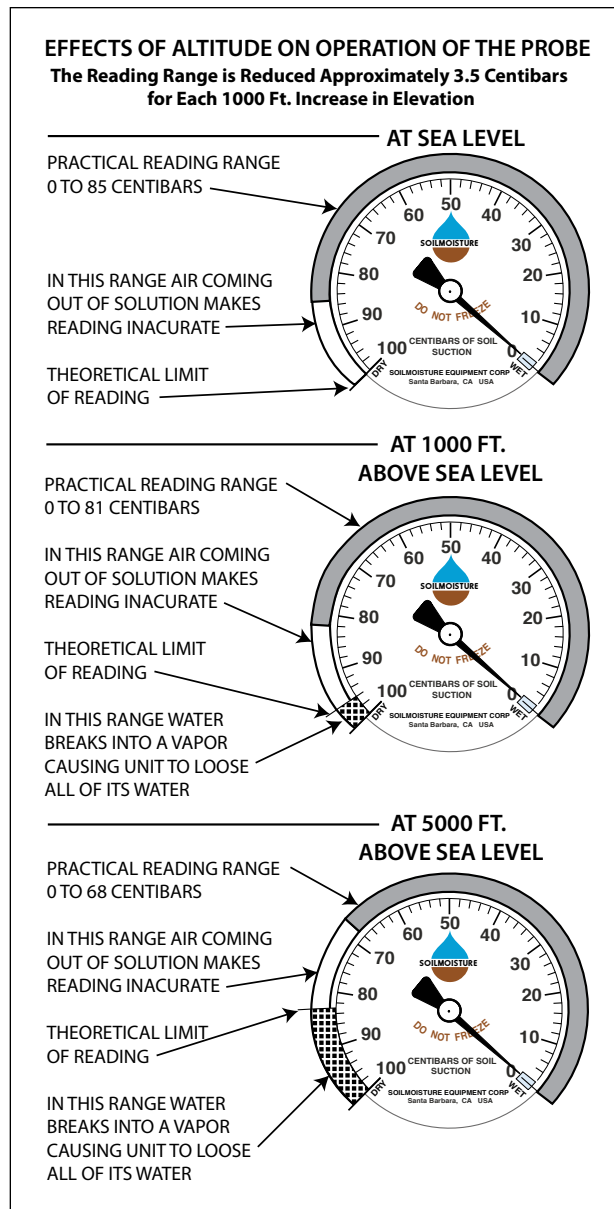
(Figure 5) - Effects of Altitude
