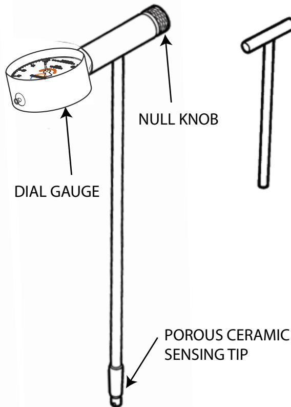
PROBE
