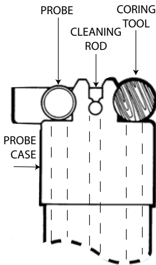
(Figure 3) - Probe case Tool placement
