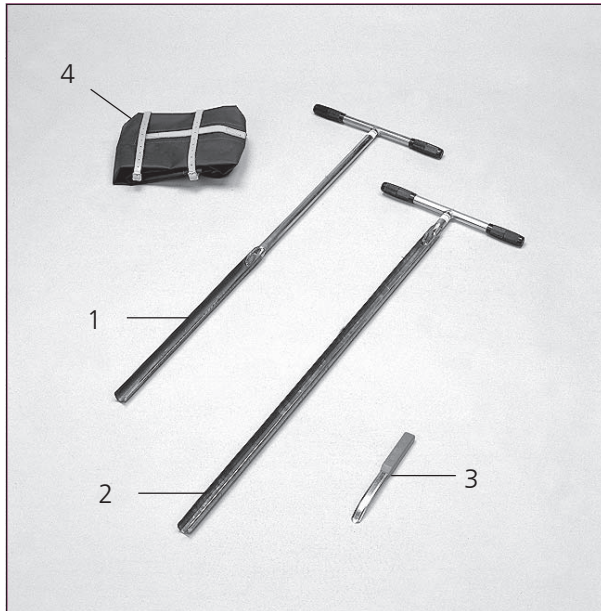
Single gouge auger set for more or less soft soils (left)
