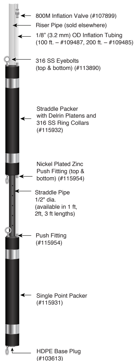
Standard Straddle Packer Setup with Inflation Lines (Inflation Tubing and Valve Not Included with Packer)
