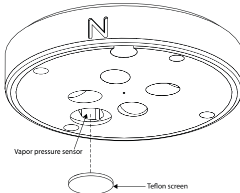
Figure 8 Vapor pressure sensor
