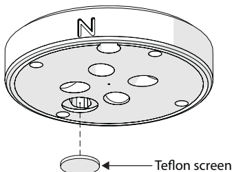
Figure 15 Teflon screen
