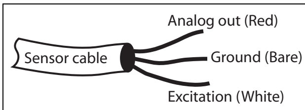
Figure 3: Sensor wiring diagram
